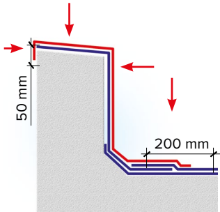
Fig. 2. Roof with torch-on application of the bottom layer
