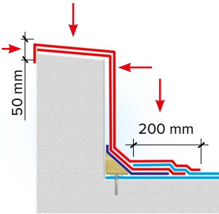
Fig. 1. Roof with mechanical fastening
